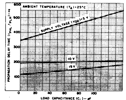
Fig. 10 — Clock-to-parallel output propagation delay vs C_L .
