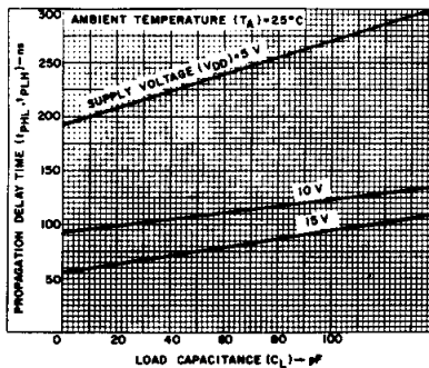
Fig. 9 — Clock-to-serial output Q_S propagation delay vs C_L .
